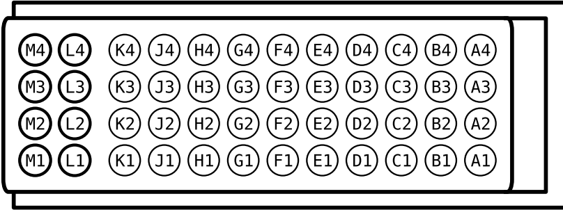
VIEWING WIRE SIDE OF LOOM PLUG
